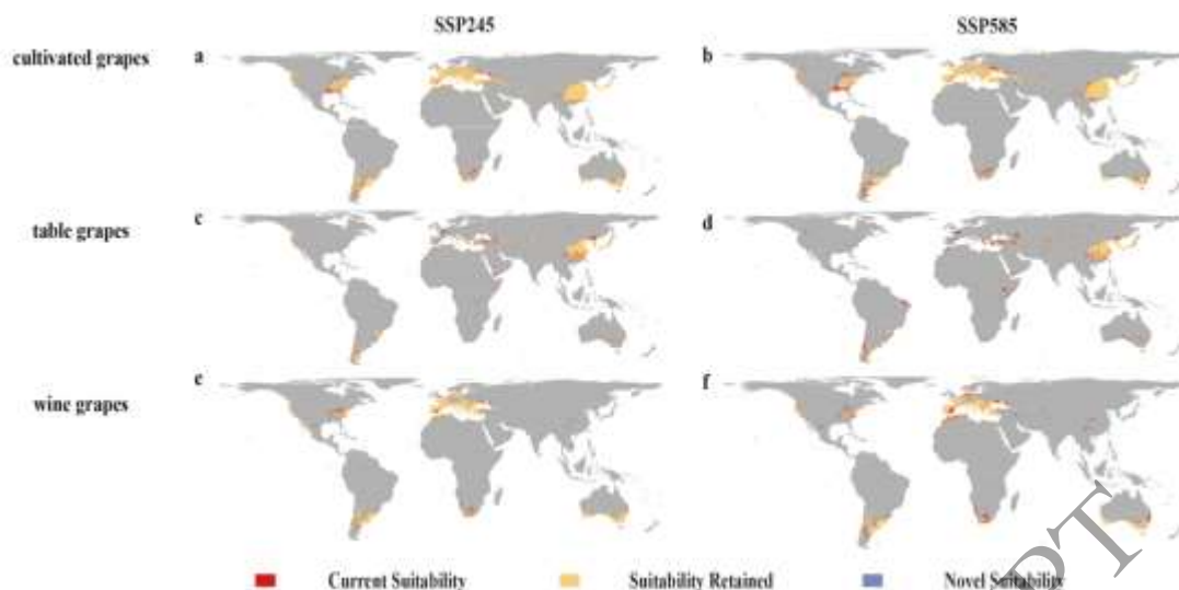
Fig. 3. Suitable distribution regions for cultivated grapes ( V. vinifera ), table grapes and wine grapes estimated using maximum entropy model; (a-b) cultivated grapes ( V. vinifera ), (c-d) table grapes, (e-f) wine grapes, with future projections for the years 2081–2100 under the SSP245 and SSP585 climatic scenarios. The projected bioclimatic suitability for Thompson Seedless and Chardonnay under the SSP245 and SSP585 scenarios can be found in the Supplementary Material (Fig. S4).
