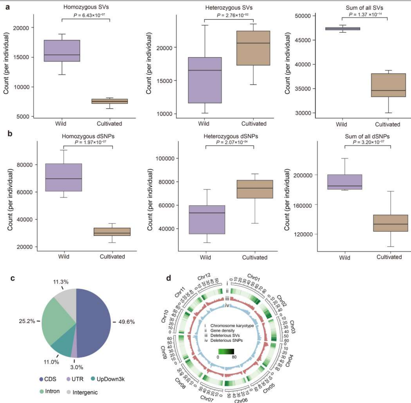
Extended Data Fig. 7 | The characteristics of SVs, dSNPs and dSVs in the potato genome. a , The number of homozygous SVs, heterozygous SVs and the sum of all SVs (twice the number of homozygous SVs plus the number of heterozygous SVs) across our panel of potato genomes. b , The number of homozygous dSNPs, heterozygous dSNPs and the sum of all dSNPs across our panel of potato genomes. For a and b , the boxes represent 75% and 25%
