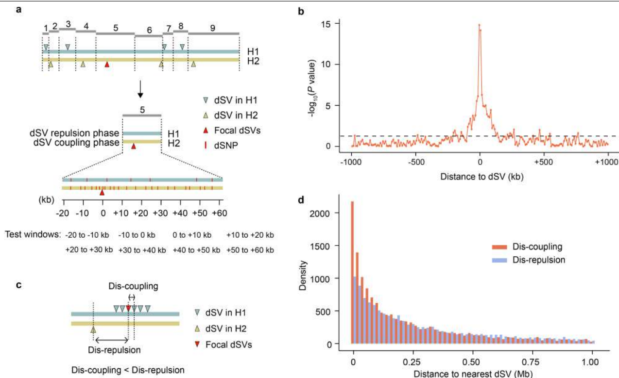
Extended Data Fig. 9 | Statistical significance of dSNP enrichment in the dSV coupling phase. a , Diagram depicting our dSNP accumulation assessment. For calculation purposes, chromosomes were segmented into fragments based on the midpoint between adjacent dSVs (irrespective whether in coupling or repulsion phase). Statistical tests were performed on each 10-kb non-overlapping window within each fragment. b , Statistical significance for the number of dSNPs flanking dSVs using the 10-kb non-overlapping windows
