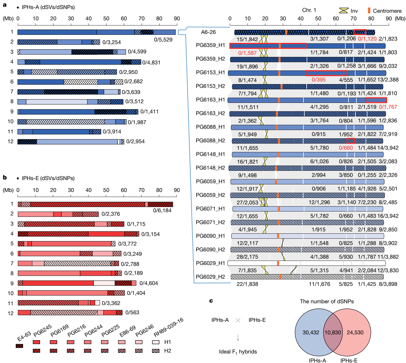
Fig. 5 | IPHs designed from the phased potato pangenome graph.
