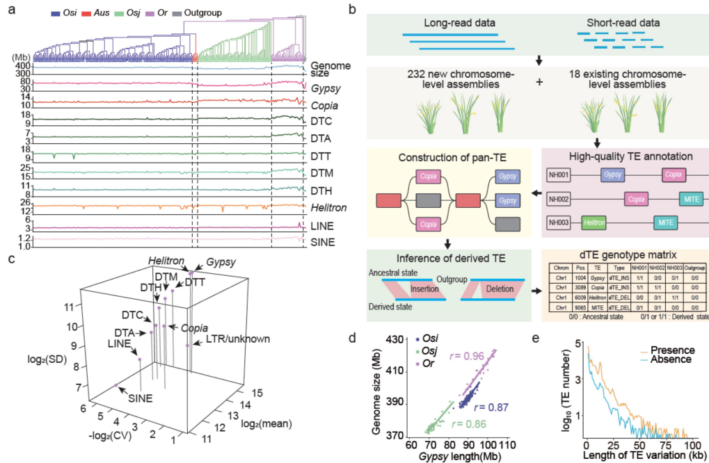
Fig. 1 Construction of a pan-TE map and evaluation of TE variations in Asian accessions using chromosome-level genomes.
