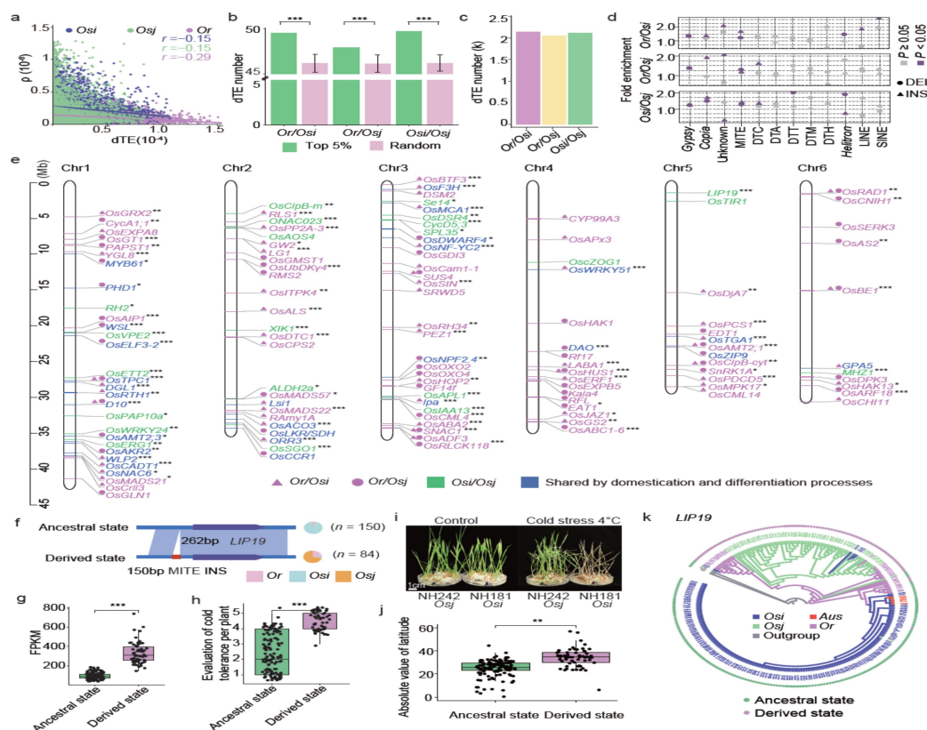
Fig. 3 Contribution of dTEs to rice domestication and differentiation.
