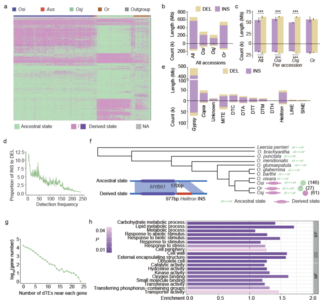
Fig. 2 Inference and characterization of TE variations representing a derived state across Asian accessions.
