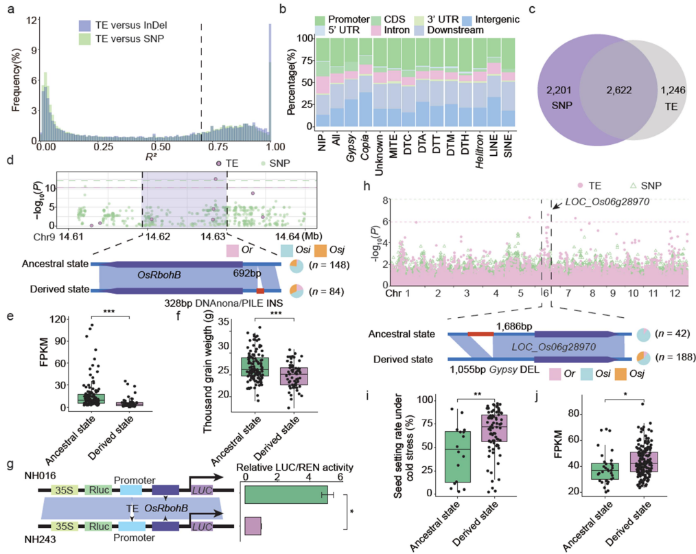
Fig. 4 TE variations associated with gene expression and agricultural traits.
