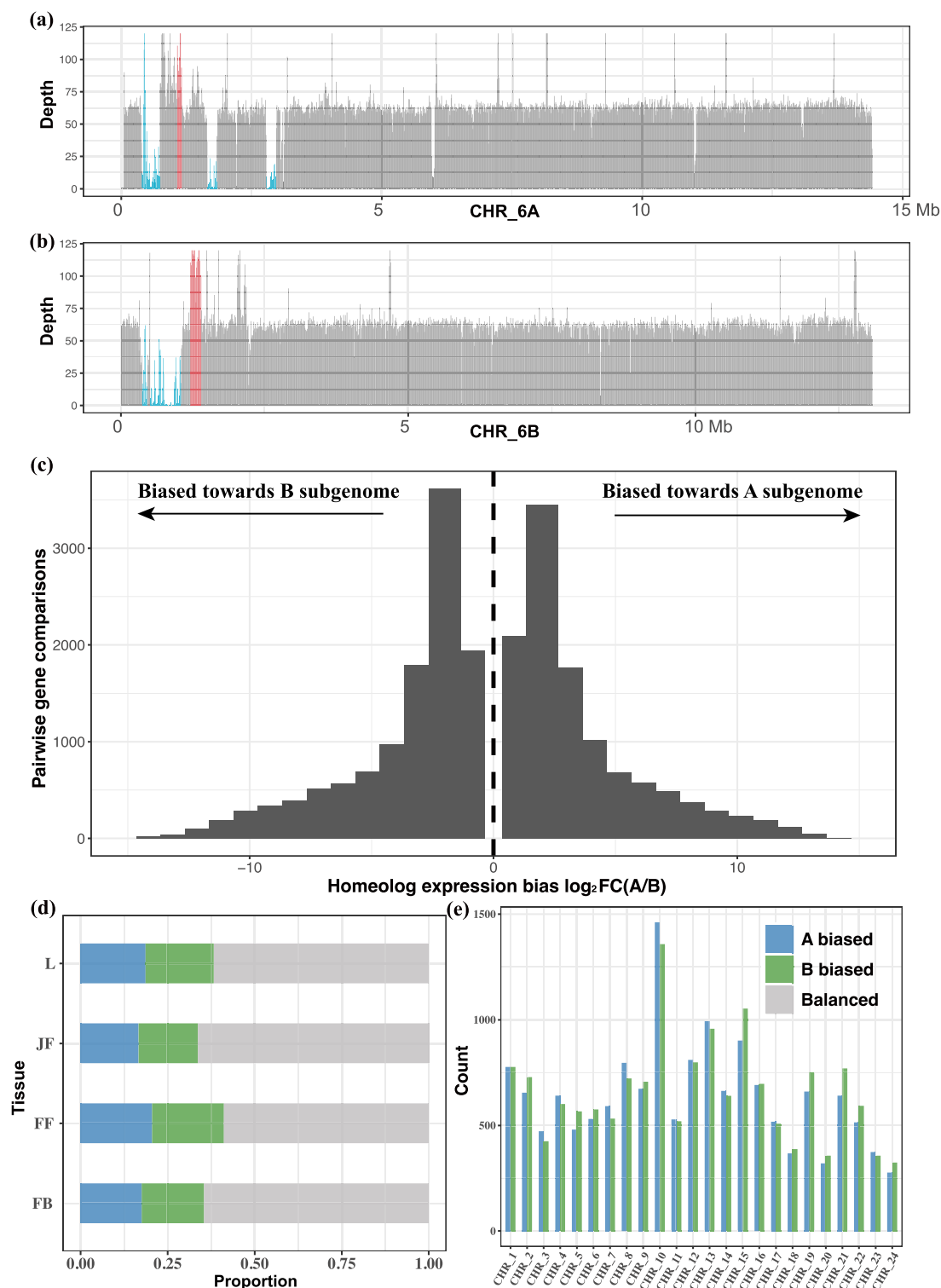
Figure 5. Homeologous exchange (HE) regions and homeologous expression bias (HBE) in the two subgenomes (TnAt vs. TnBt) of allotetraploid Trapa natans ( 2n = 4x = 96 ). (a) and (b) HE regions, as exemplified for one chromosome each of the TnAt and TnBt subgenomes. Coverage depth was obtained for CHR_6At (a) and CHR_6Bt chromosomes (b) after mapping Illumina sequence reads from allotetraploid T. natans on the diploid T. natans and T. incisa genome assemblies concatenated together. The regions with red lines represent windows whose coverage depth was 1.5 times greater than the whole-genome average depth, while the blue lines show deletions with low or no coverage. (c) Histograms of genome-wide expression of syntenic homeologous genes among the TnAt and TnBt subgenomes. (d) and (e) Pairwise comparisons between syntenic gene pairs among four tissues (FB: flower bud; FF: fertilized flower; JF: juvenile fruit; L: leaf) (d) and among the 24 chromosome pairs (e) .
